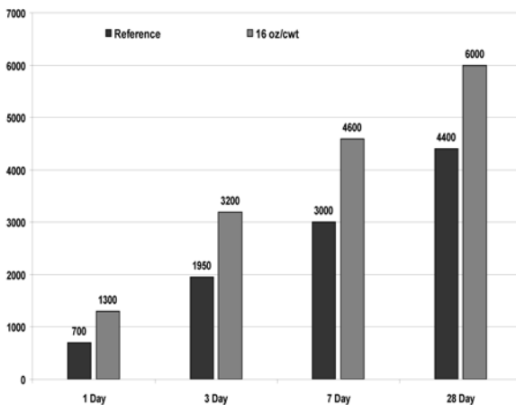
Eucon 37 Compressive Strength Results (psi)
